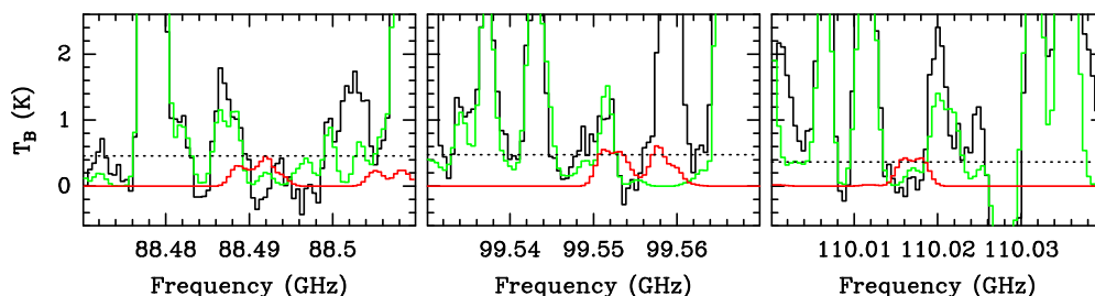
Fig. 1. Synthetic LTE spectrum of thioacetaldehyde (in red) used to derive the upper limit to its column density, overlaid on the ALMA spectrum of Sgr B2(N2) (in black) and the synthetic spectrum that contains the contributions of all the species (but not thioacetaldehyde) that we have identified so far in this source on the basis of the EMOCA survey (in green). The dotted line in each panel indicates the 3\sigma noise level. Other transitions of thioacetaldehyde that are expected to be weaker than 3\sigma and/or heavily contaminated by other species are not shown. (For interpretation of the references to colour in this figure legend, the reader is referred to the web version of this article.)
